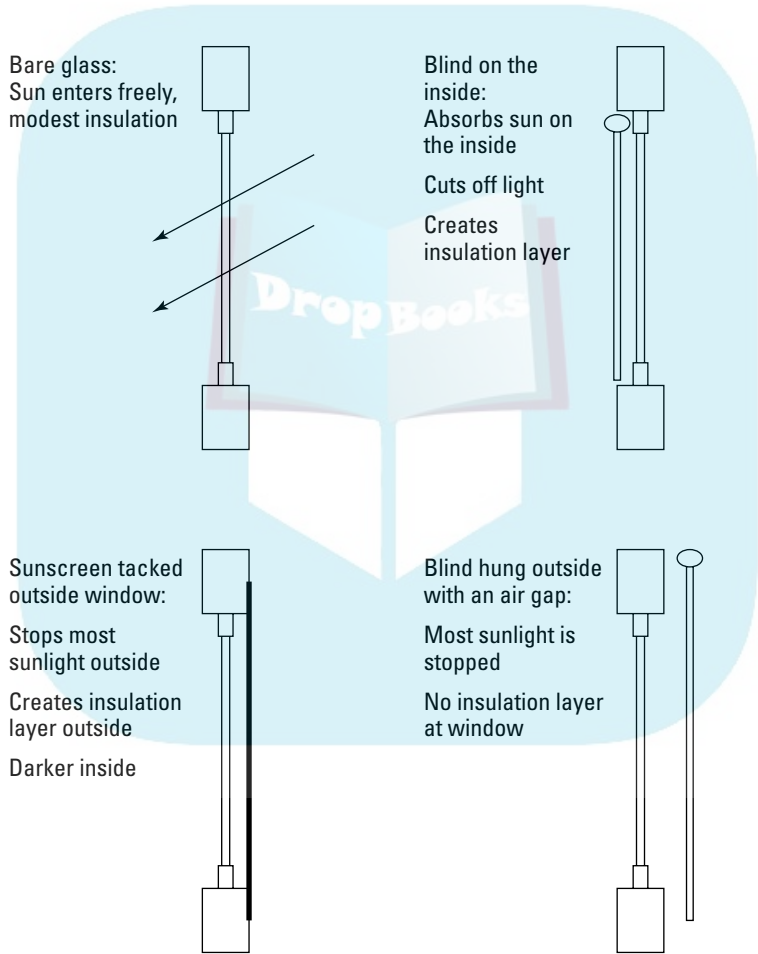
Figure 9-1: Differences in the ways to cover a window.
